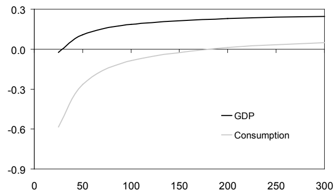
Figure 8 Welfare vs elasticity of demand
